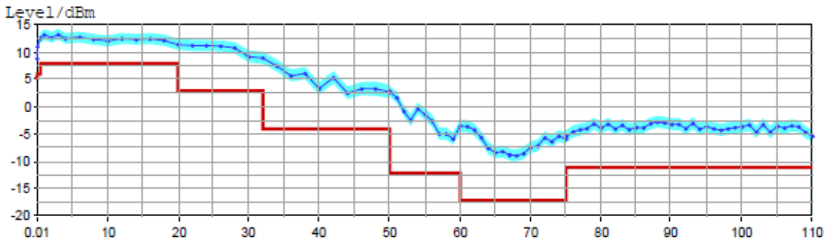
Maximum output power in dBm versus frequency in GHz of the R&S ® ZVA110.
